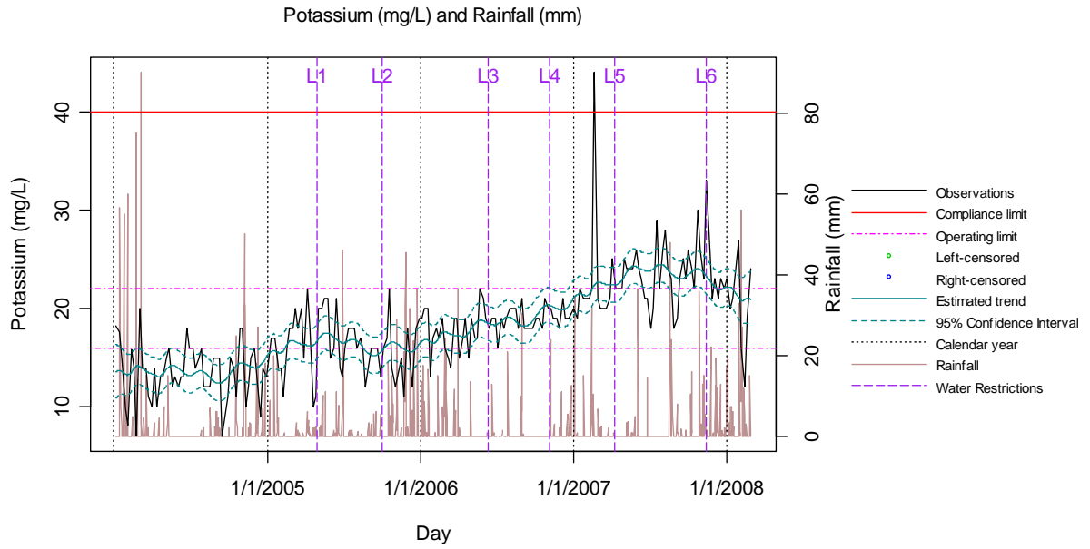
Figure 31 Plot of Effluent Potassium Levels Recorded at Bundamba WWTP
