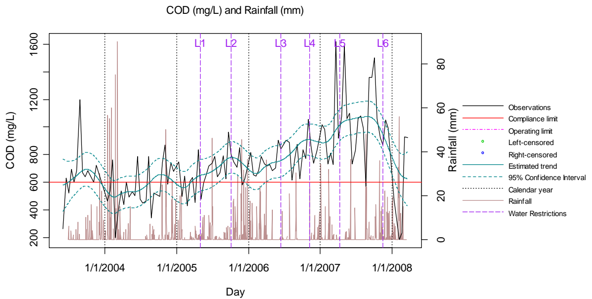
Figure 10 Observed COD Values at the Inlet of the WWTP
