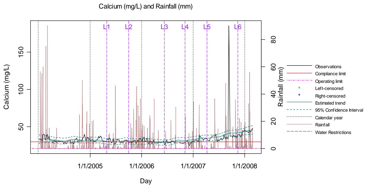
Figure 32 Plot of Effluent Calcium Levels Recorded at Bundamba WWTP
