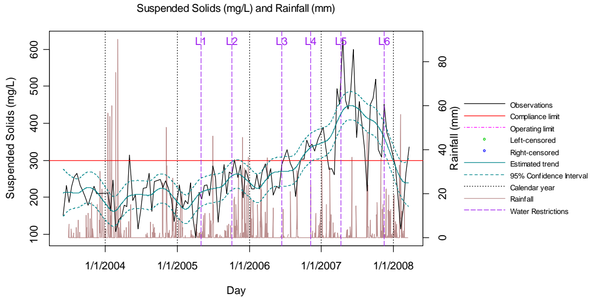
Figure 9 Observed Suspended Solids Values at the Inlet of the WWTP
