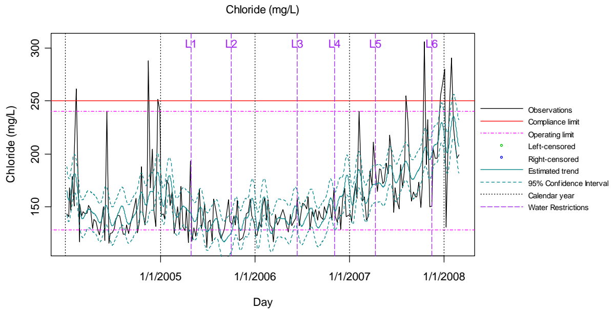
Figure 26 Plot of Effluent Chloride Levels Recorded at Bundamba WWTP
