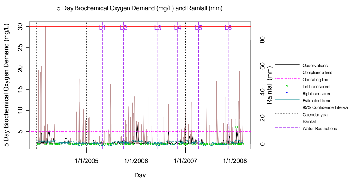
Figure 21 Plot of Effluent BOD 5 Values Recorded at Bundamba
