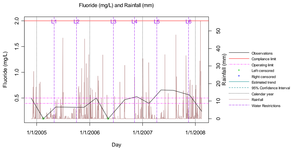
Figure 27 Plot of Effluent Fluoride Levels Recorded at Bundamba WWTP
