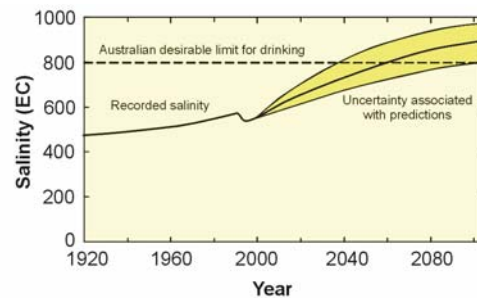
Figure 18. Salinity of the River Murray at Morgan in South Australia. (Source: MDBC 6 .)
