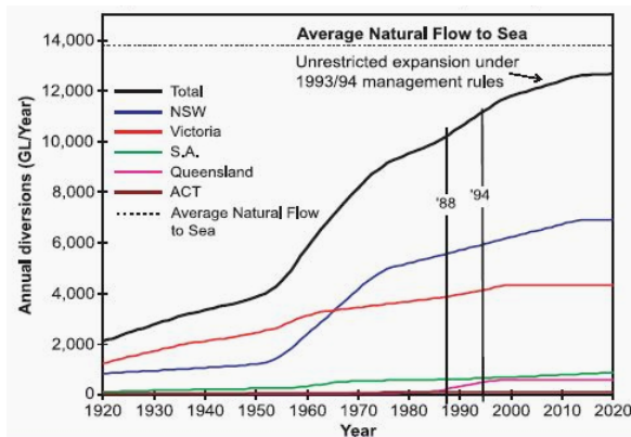
Figure 19. Water use and the Cap. (Source: Crabb 12 .)
