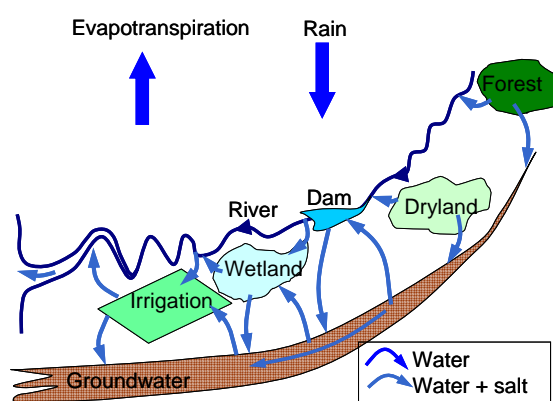
Figure 1. Schematic representation of water resource movement patterns in the Basin.
