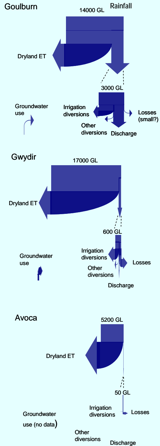
Figure 17. Approximate catchment water flows for Gwydir, Goulburn and Avoca, based mainly on SILO rain datasets 10 , water audit monitoring reports 1 , and river gauging data from the New South Wales Pineena database 14 and the Victorian Water Data Warehouse 16 . Losses were too small to estimate reliably for Goulburn.
