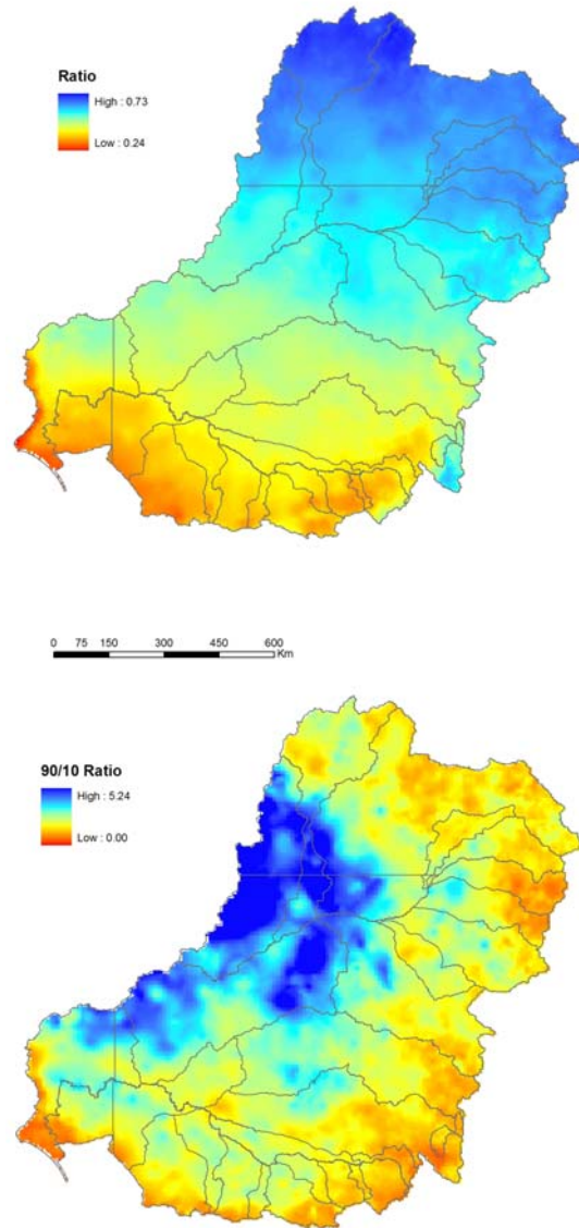
Figure 3. Summer rainfall dominance (proportion of rain falling in summer, top) and variability (ratio of 90 to 10 percentile rain, bottom). (Source: SILO datasets 11 .)
