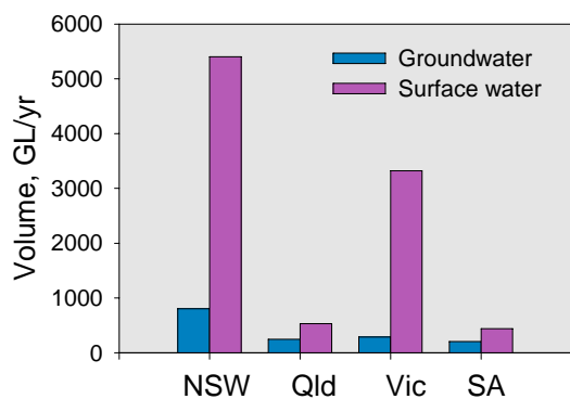
Figure 14. Use of groundwater and surface water by State. (Source: Evans et al. 27 .)
