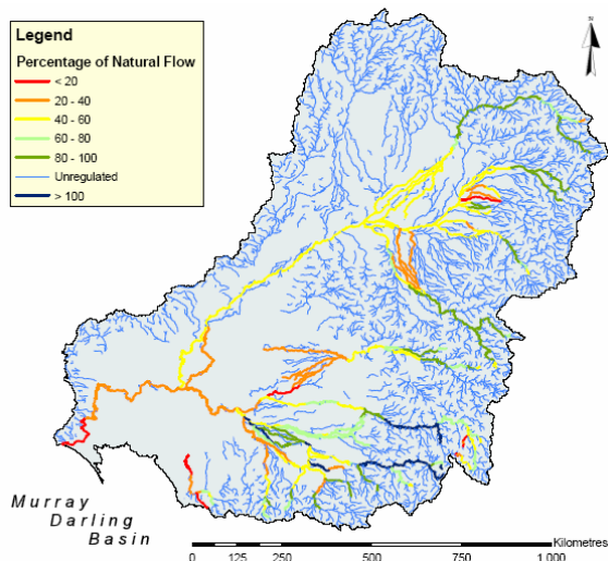
Figure 10. Regulated river links showing the proportion of flow lost at reservoirs or off-takes and gains due to releases from hydroelectric schemes and some irrigation canal inflow. (Source: DeRose et al. 18 .)
