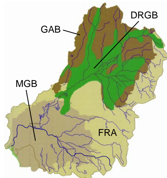
Figure 12. General distribution of the Great Artesian Basin (GAB), Murray Groundwater Basin (MGB), the Darling Regional Groundwater Basin (DRGB) and fractured rock aquifers (FRA) (Source: Breckwoldt et al. 13 .)
