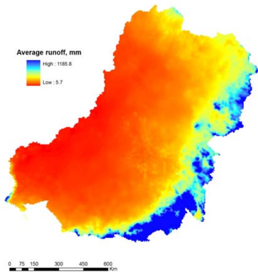
Figure 5. Annual average run off, calculated as the difference between rainfall and actual evapotranspiration (Source: SILO datasets 2.)
