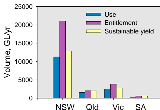
Figure 15. Summary of groundwater use, yield and allocation, by State in 2002-03. (Source Evans et al. 27 .)
