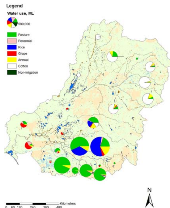
Figure 11. Major irrigation water uses (estimated) by sub-catchment in the Murray-Darling Basin (Source: based on Bryan and Marvanek 23 ).
