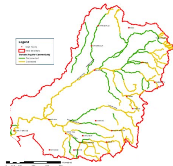
Figure 13. Connected and disconnected rivers in the Murray-Darling Basin. Some reaches may alternate between connected and disconnected in greater detail than shown. (Source: Evans et al. 27 .)
