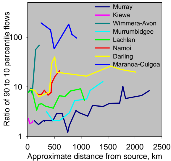
Figure 6. Variation in annual flow (ratio of 90th to 10th percentile flows) as a function of distance from source. (Source: New South Wales Pineena database 14 , Watershed in Queensland 15 and the Victorian Water Data Warehouse 16 .)
