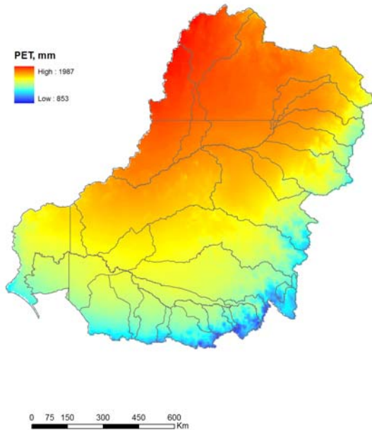
Figure 4. Potential evapotranspiration. (Source: SILO datasets 2,11 .)
