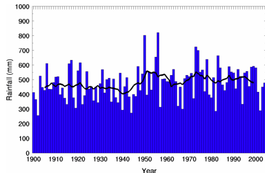
Figure 3. Annual precipitation across the Basin. The line shows the 11-year moving average. (Source: Bureau of Meteorology 7 )
