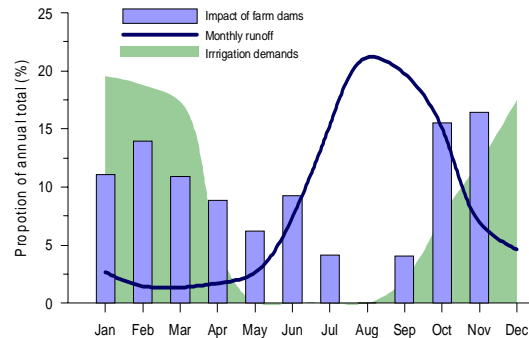
Figure 29. Typical pattern of irrigation demands and impacts for a catchment located in south-eastern Australia. (Source: SKM, 2004 44 )
