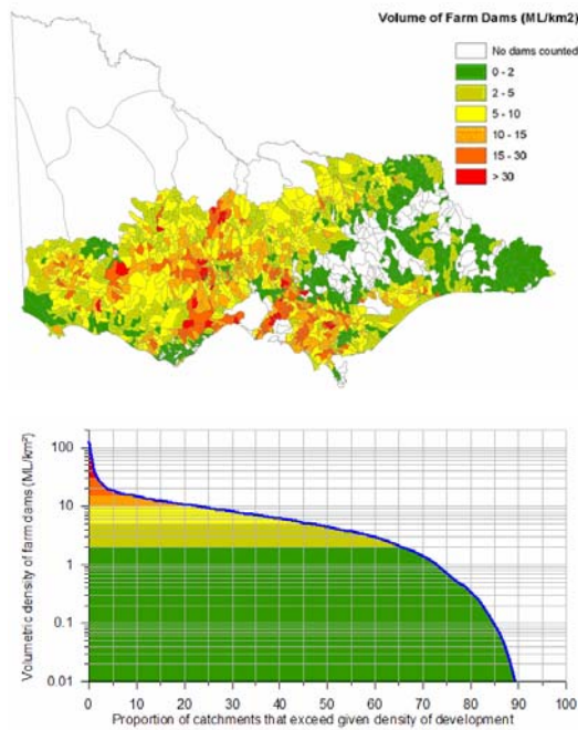
Figure 26. Map and summary of distribution of farm dam development in Victoria. (Source: Lowe et al. 34 )
