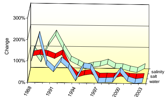
Figure 13. Annual values of stream flow, salt load and stream salinity for Pine Creek (a very small 3 km 2 catchment in the southwest Goulburn River catchment, Victoria) after full afforestation was completed in 1988. (Source: Harisine & Van Dijk 22 )
