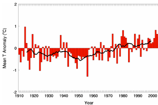
Figure 2. Annual anomalies (based on 1961-1990 averages) of mean temperature in the Basin. The line shows the 11-year moving average. (Source: Bureau of Meteorology 7 )
