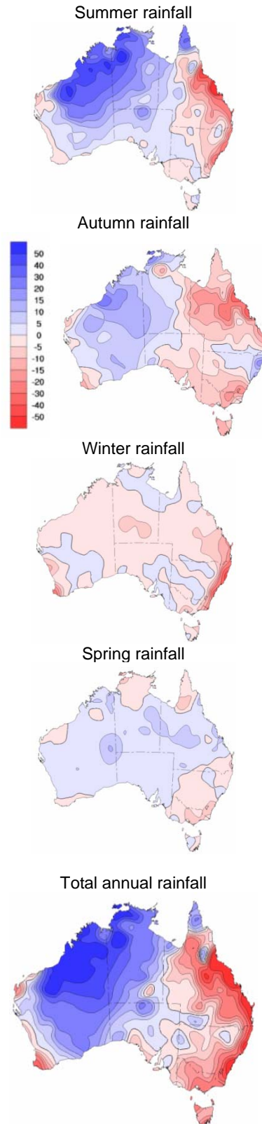
Figure 4. Observed trends in seasonal and annual rainfall the period 1950–2004. Units are the rate of change in millimetres per decade. (Source: Bureau of Meteorology 7 .)
