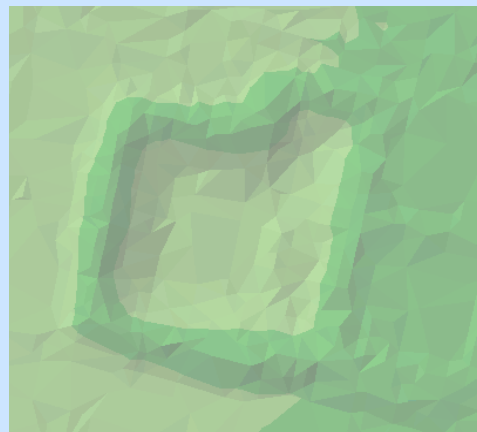
Figure 27. Example of a high resolution digital model of a dam.
